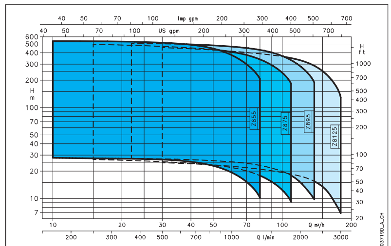
Characteristic curves of 50 Hz Z8-ZR8 Series.
